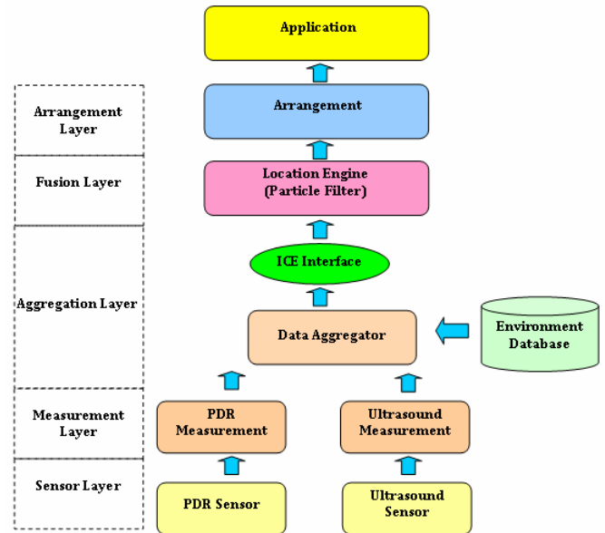
Fig. 4. Block Diagram of localization system and corresponding layer in the localization model
